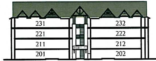
FRONT ELEVATION: PARKING LOT SIDE
