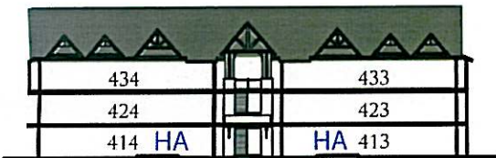
REAR ELEVATION: INTERIOR SIDE
